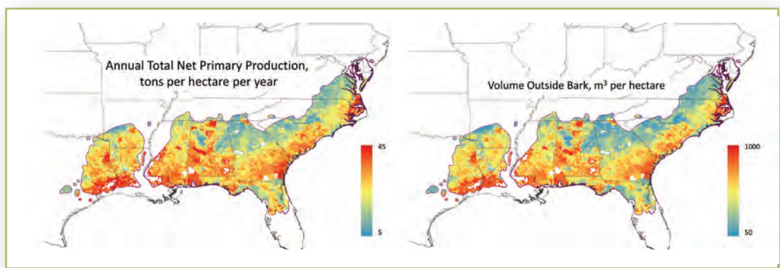
Figure 6.2. Example outputs from 3-PG. The natural range of loblolly pine is outlined in purple.
