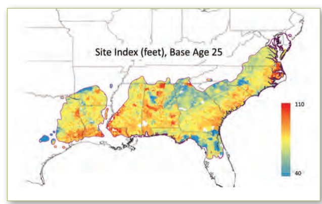
Figure 6.1. SSURGO-derived site index for the PINEMAP region. The natural range of loblolly pine is outlined in purple.
